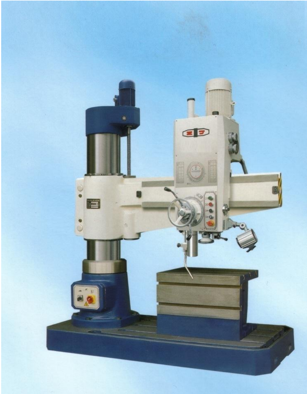
SAMSTAR MODEL #Z3050xI6/1 63" X 13 3/4" RADIAL DRILL
